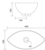
BRAVIA Table Top Basin 600x360x120mm 24"x14"x5" 6.60 Kg.
